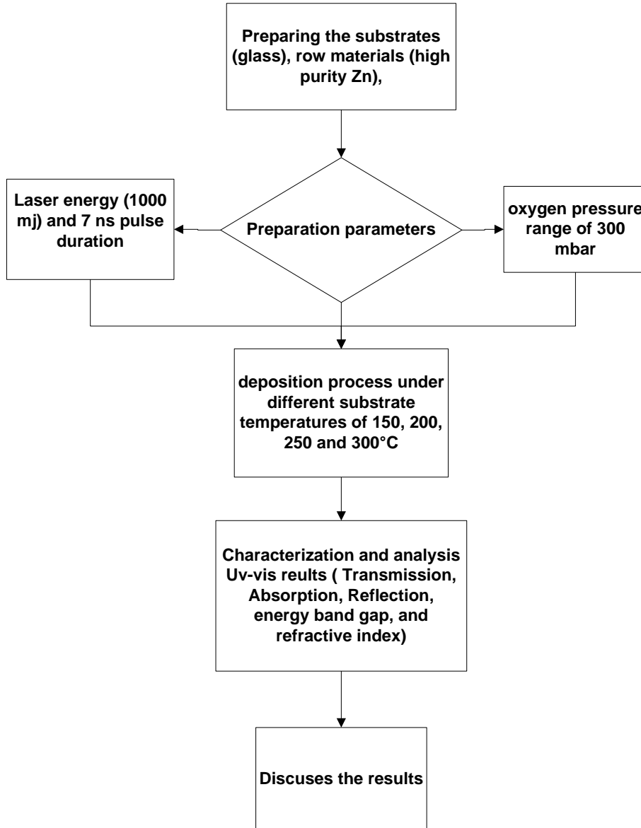
Figure 1. Flowchart of the ZnO nano thin Film preparation process
