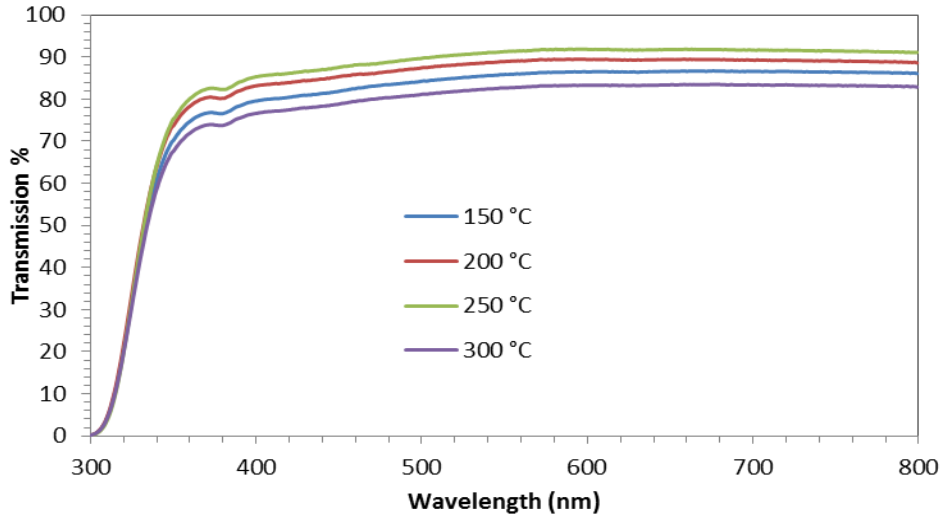
Figure 2. The Transmission curve as a function of the wavelength ranges between 300 nm to 800 nm.
