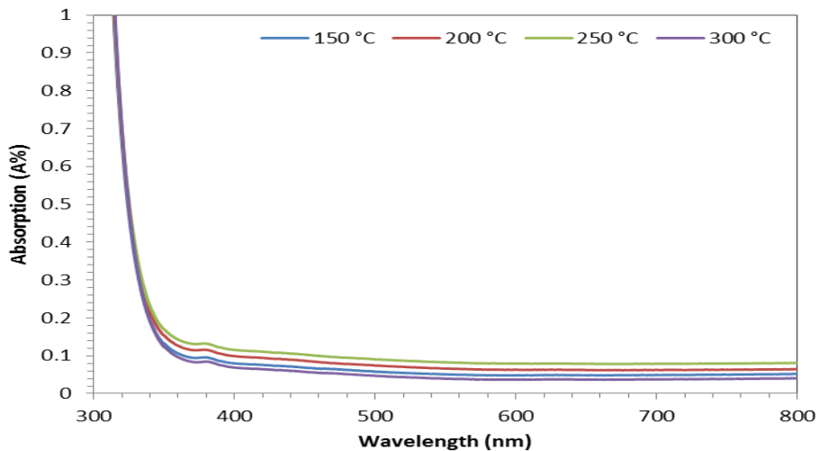
Figure 3. Optical absorption curve as a function of wavelengths under two substrate temperatures.
