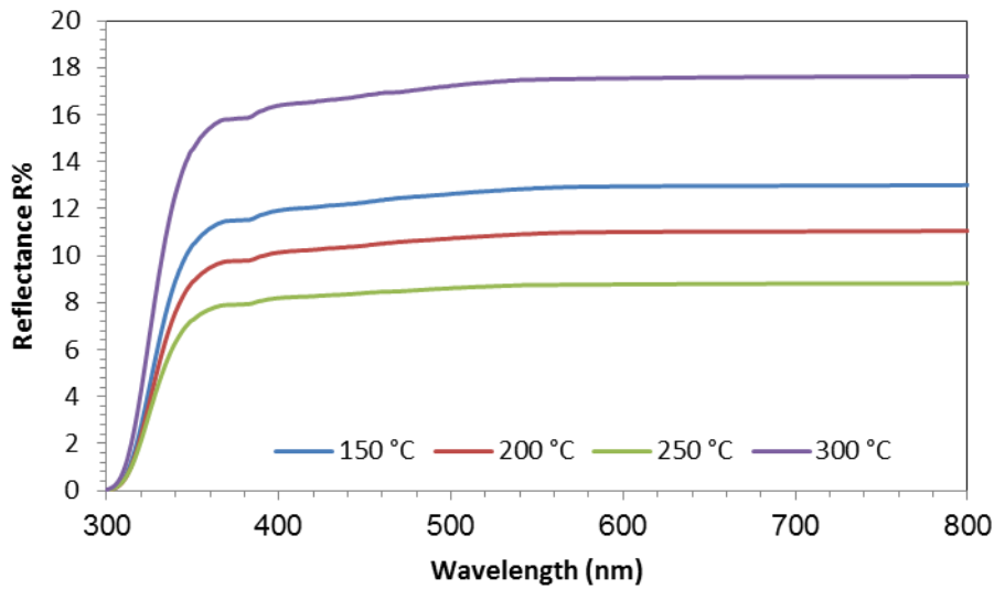
Figure 5. Reflectance as a function of wavelength range under two substrate temperatures
